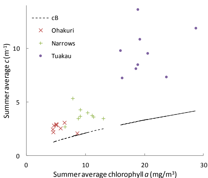
Figure 5: Summer-average chlorophyll a and beam attenuation at three Waikato River sites during 2005–14 (summer: October-to-March). The dashed line shows the upper bound to the contribution of phytoplankton to attenuation (as c_B = 0.47 \times [\text{Chlorophyll } a]^{0.65} ; see text).
