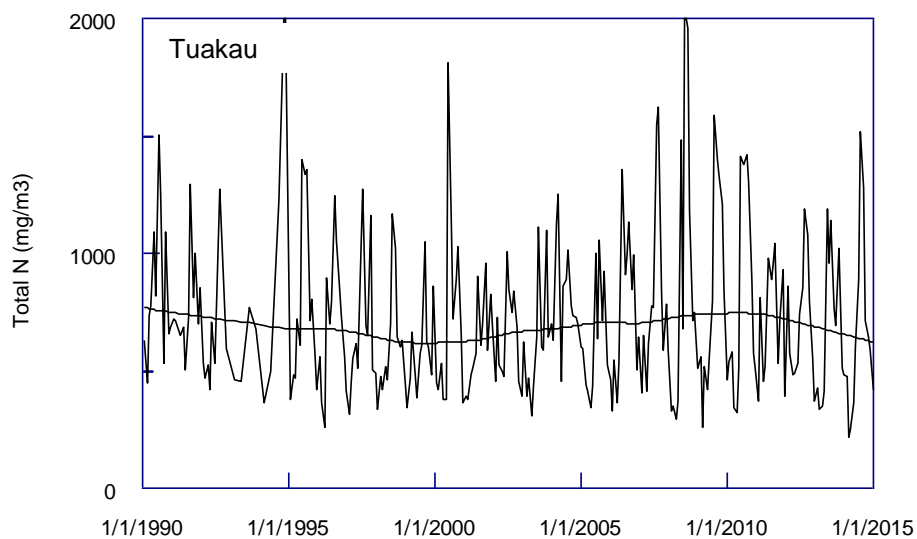
Figure A2: Monthly measurements of total nitrogen in the Waikato River at Ohakuri, Narrows and Tuakau, 1990–2014. LOWESS smoothing curves have been fitted to the data.
