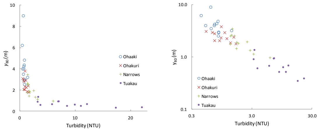
Figure 2: Black disc sighting range ( y_{BD} ) and turbidity in monthly samples from four sites on the Waikato River, January-December 2014. Results are plotted on both normal axes (left) and logarithmic axes (right).
