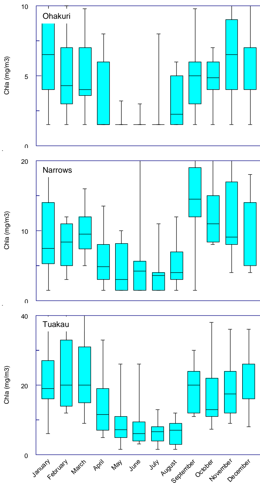
Figure 4: Seasonal boxplots of chlorophyll a concentration at selected sites on the Waikato River, 2005–14
