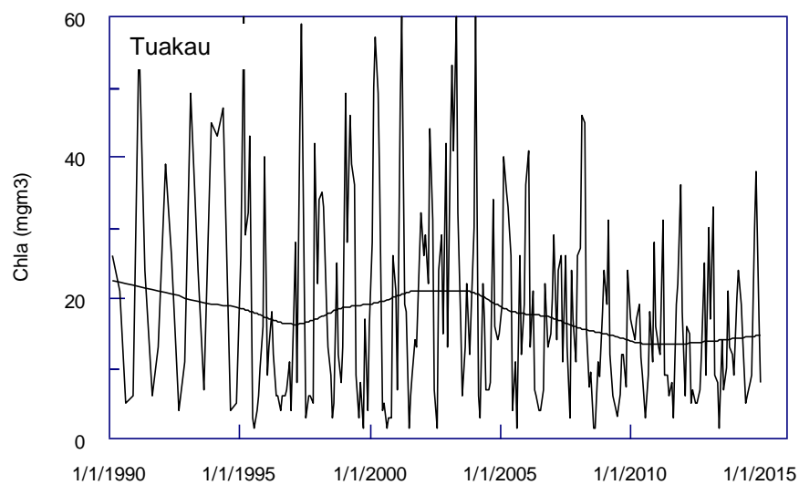
Figure 8: Monthly measurements of chlorophyll a in the Waikato River at Ohakuri, Narrows and Tuakau, 1990–2014. LOWESS smoothing curves have been fitted to the data.
