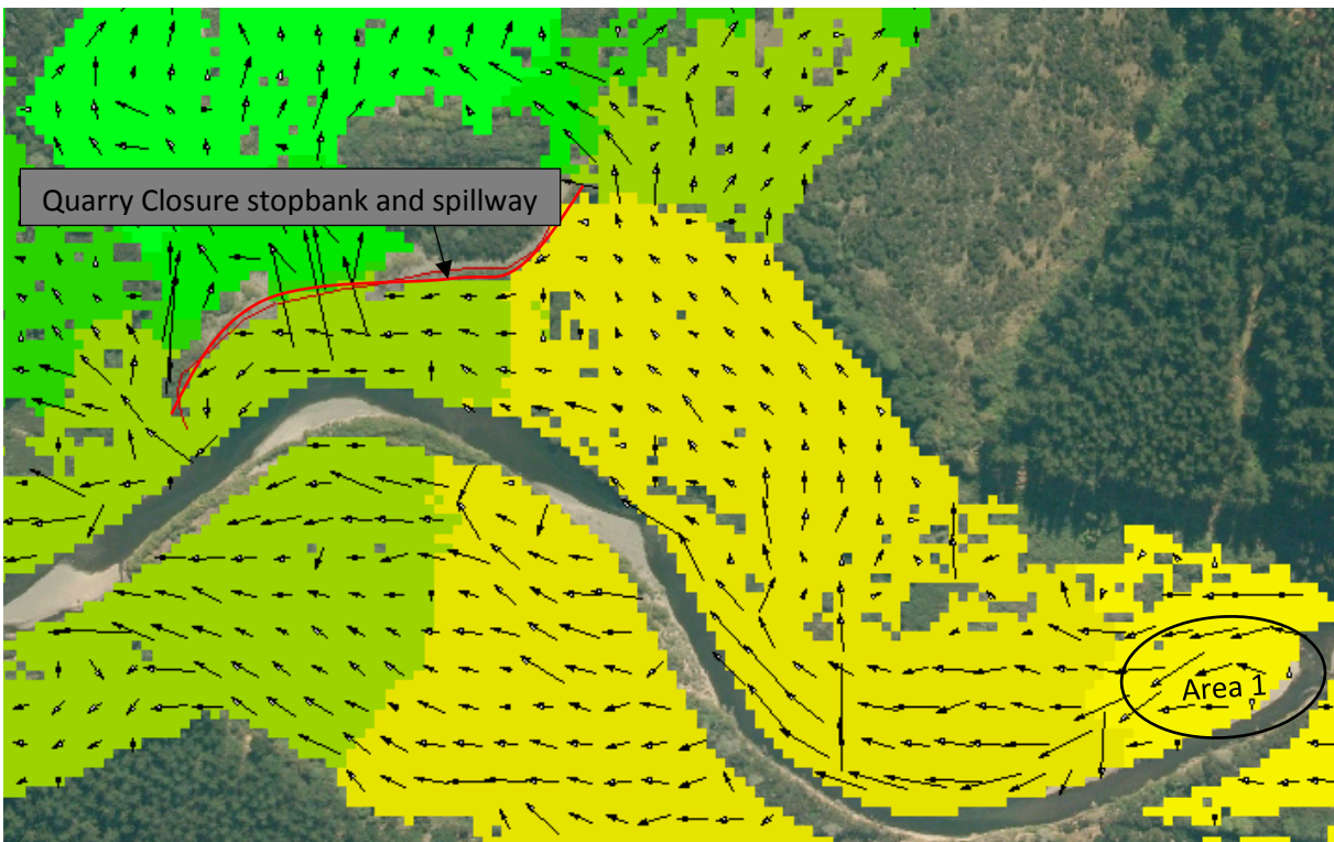
Quarry Closure Stopbank and upstream area – flow vectors
